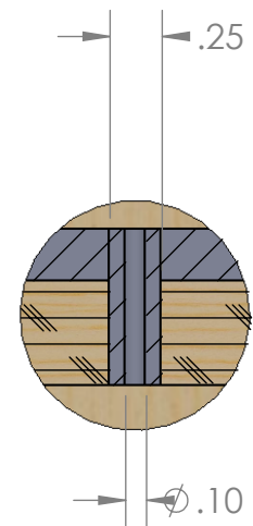
DETAIL C SCALE 1 : 1
